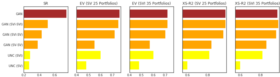
Figure 4: GAN Illustration
