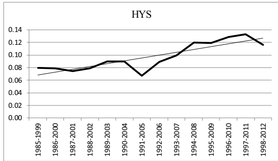
(a) HYS
