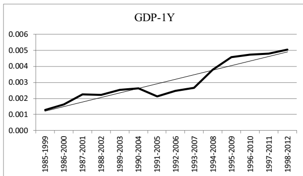
(c) GDP
